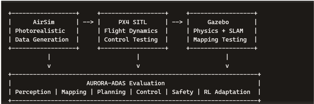
Fig. 12. Simulation and evaluation pipeline for AURORA-ADAS. The diagram illustrates the integrated multi-environment simulation workflow used to develop, validate, and benchmark the AURORA-ADAS autonomy stack. AirSim provides photorealistic rendering and multi-modal data generation for perception training, including RGB, depth, and semantic labels. PX4 SITL offers high-fidelity flight dynamics and real-time control testing through MAVLink offboard
