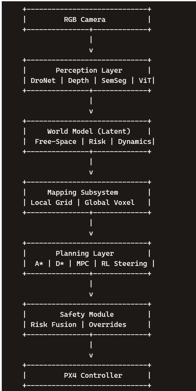
Fig. 3. Layered methodology architecture of the AURORA-ADAS autonomy system. The diagram illustrates the hierarchical flow of information from raw sensor inputs to final motor commands. RGB imagery is processed through a multi-branch perception layer consisting of
