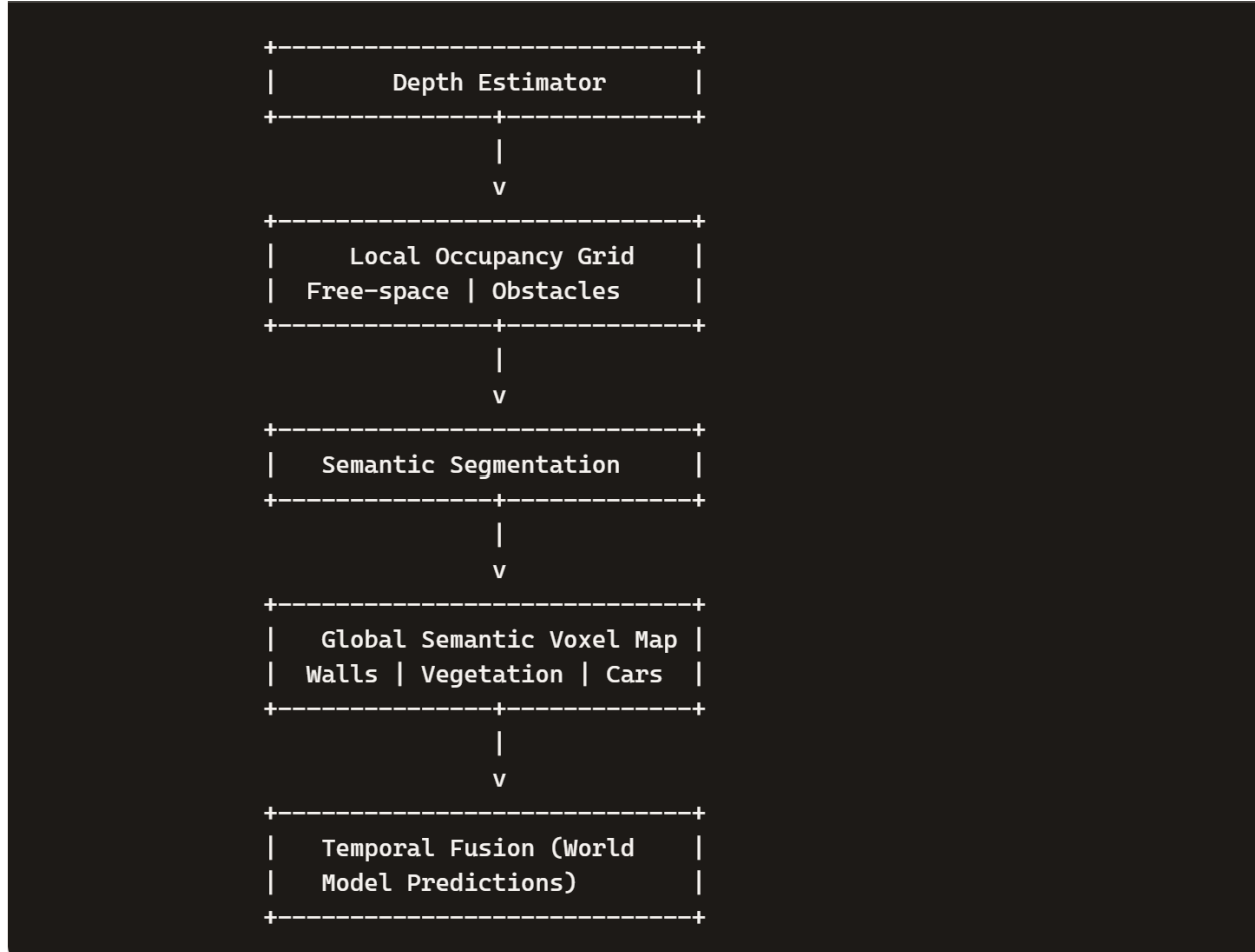
Fig. 9. Deep mapping architecture integrating geometric, semantic, and temporal scene understanding in AURORA-ADAS. The diagram illustrates the hierarchical mapping pipeline that transforms raw depth and semantic information into rich spatial representations for navigation. Depth estimation produces geometric structure that is converted into a local occupancy grid encoding free-space and obstacles. Semantic segmentation provides pixel-wise class labels that are fused into a global semantic voxel map, enabling the system to distinguish between structural elements such as walls, vegetation, and vehicles. Temporal fusion incorporates predictions from the world-model subsystem, combining free-space forecasts and obstacle-motion dynamics with the geometric and semantic maps. This multi-layered mapping framework yields a unified, temporally consistent representation of the environment, supporting robust planning and safety-aware decision-making in GNSS-denied conditions.
